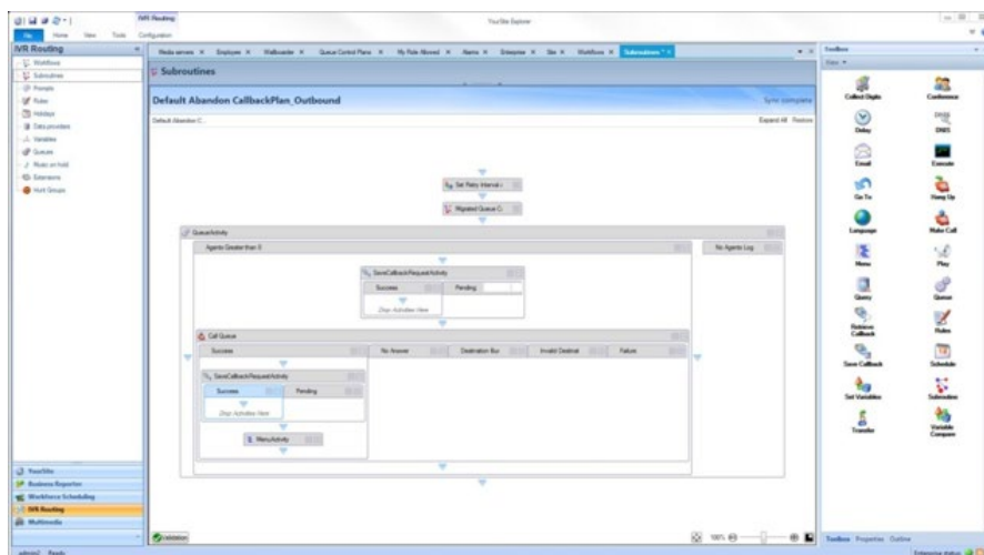
Mitel IVR designer, call-flow and toolbox
